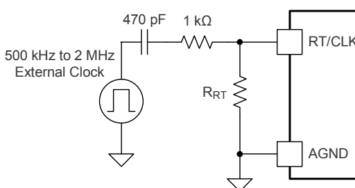
Figure 28. CLK/RT Configuration
